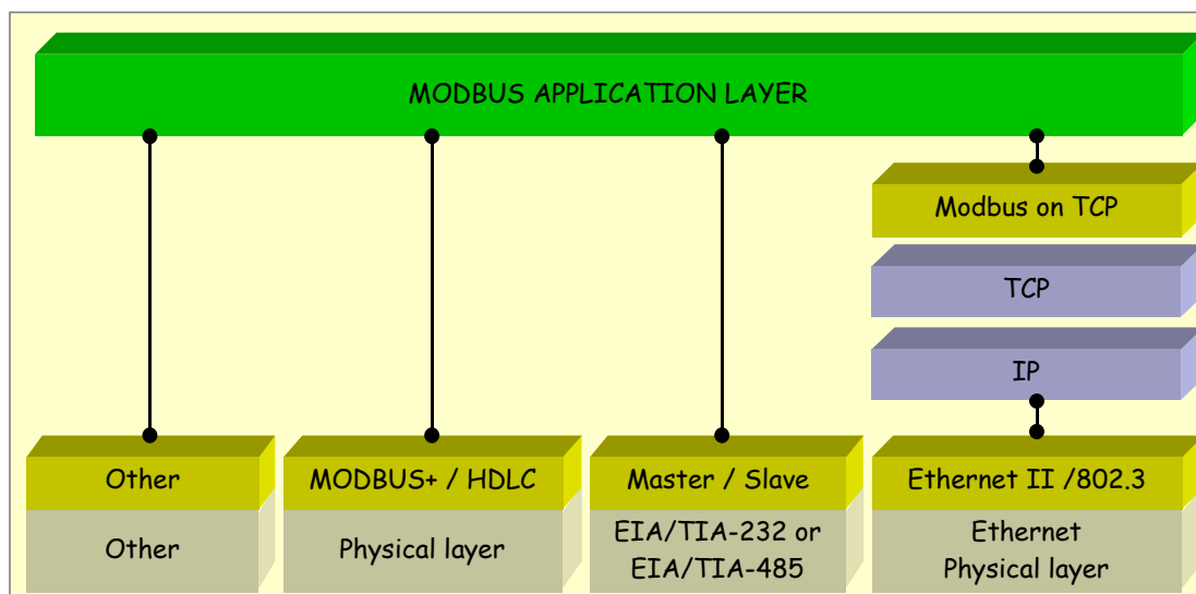
Figure 1: MODBUS communication stack
